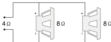
Parallel wiring
