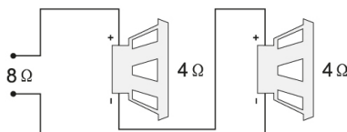
Series wiring
